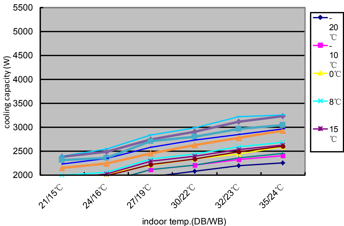
cooling capacity and indoor/outdoor temp.curves
